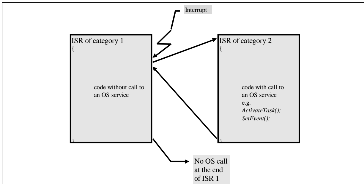
Figure 14-1 Nested interrupts
