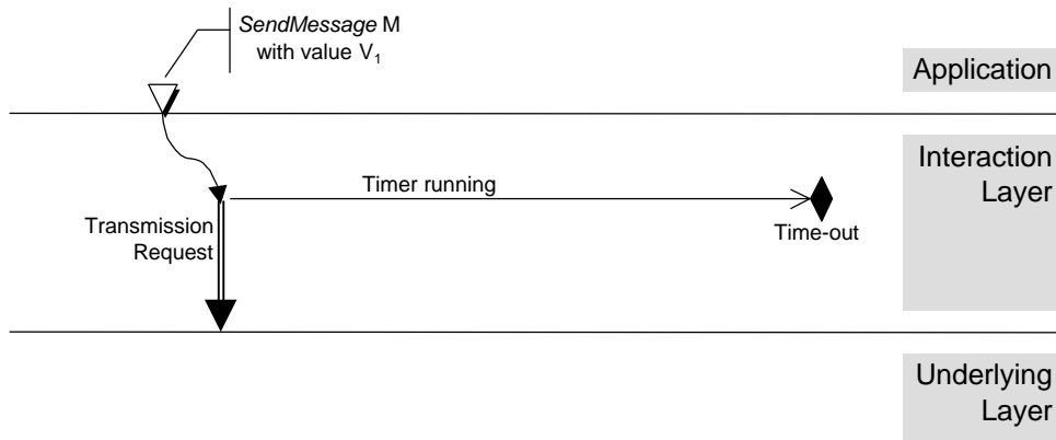
Figure 2-13: Direct Transmission Mode: example of a failed transmission
